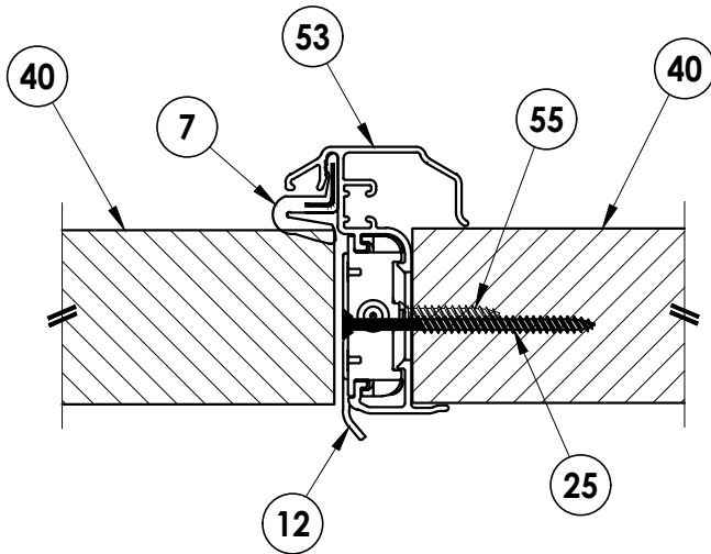
1 7 HORIZONTAL CROSS SECTION Outswing Shown (Inswing Similar)
