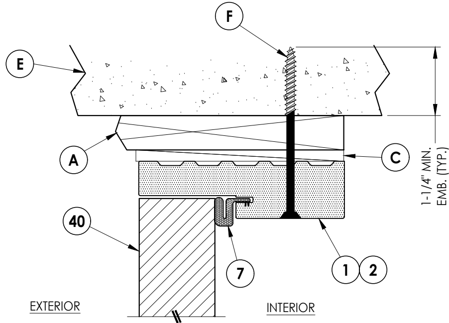
3 9 VERTICAL CROSS SECTION Outswing Shown (Inswing Similar) Shown w/ 1X Buck
