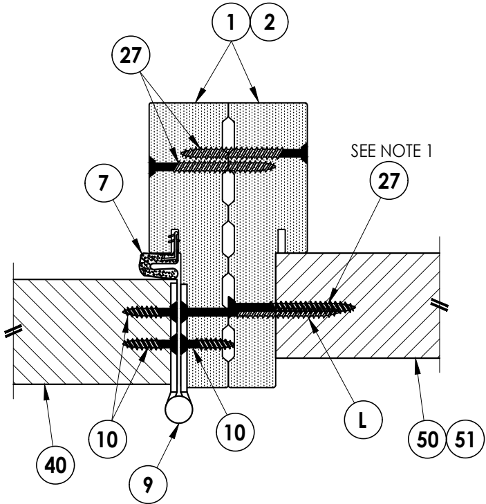
2 7 HORIZONTAL CROSS SECTION Outswing Shown (Inswing Similar)
