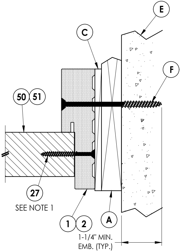
2 9 HORIZONTAL CROSS SECTION Outswing Shown (Inswing Similar) Shown w/ 1X Buck
